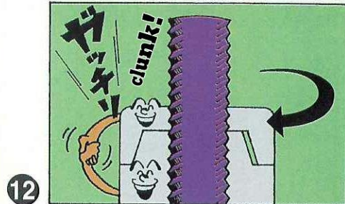
12 What's more, the Hard Lock Nut pushes in the wedge using a bolt screw, so the fastening work can be done with a minimum of force. And of course, removal is easy too.
