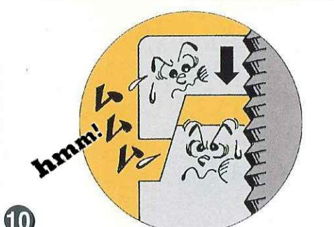
10 Look at this cross-sectional view. Here, the lower nut (A) is carrying out the wedge role. When (A) is pushed into the space of the upper nut (B), a wedge effect is exhibited. This results in a powerfully locked condition.
